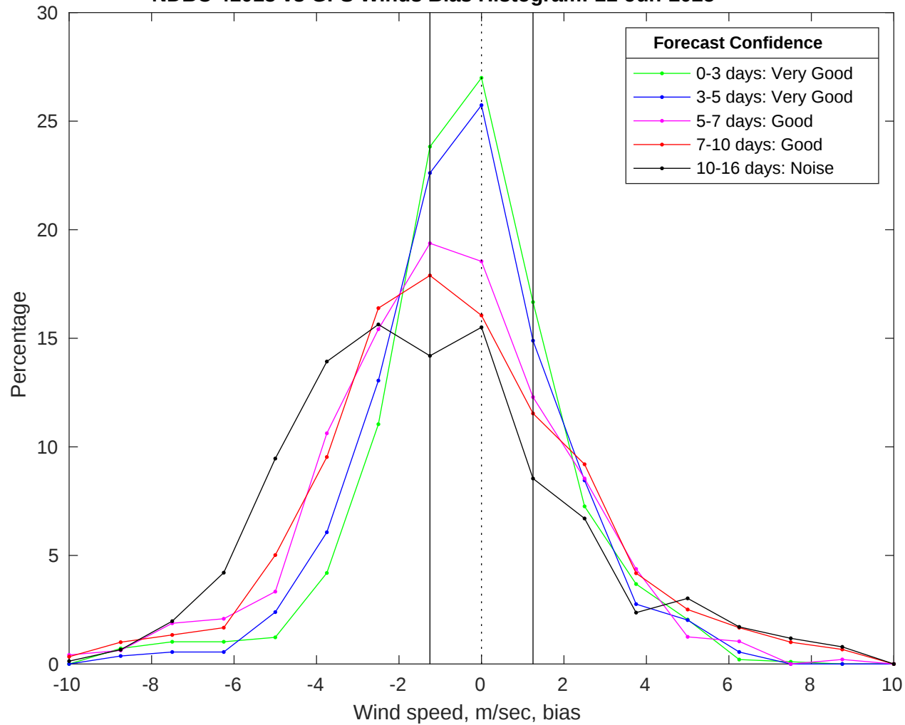
NDBC 41013 vs GFS Winds Bias Histogram: 11-Jun-2025
