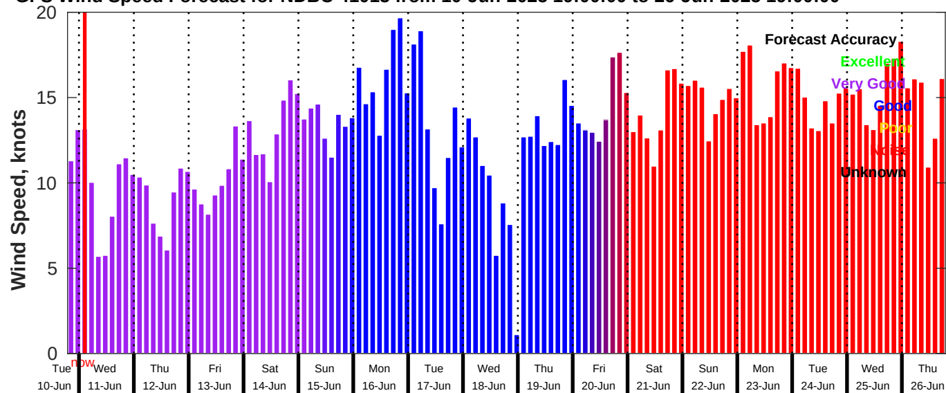
GFS Wind Speed Forecast for NDBC 41013 from 10-Jun-2025 19:00:00 to 26-Jun-2025 19:00:00
