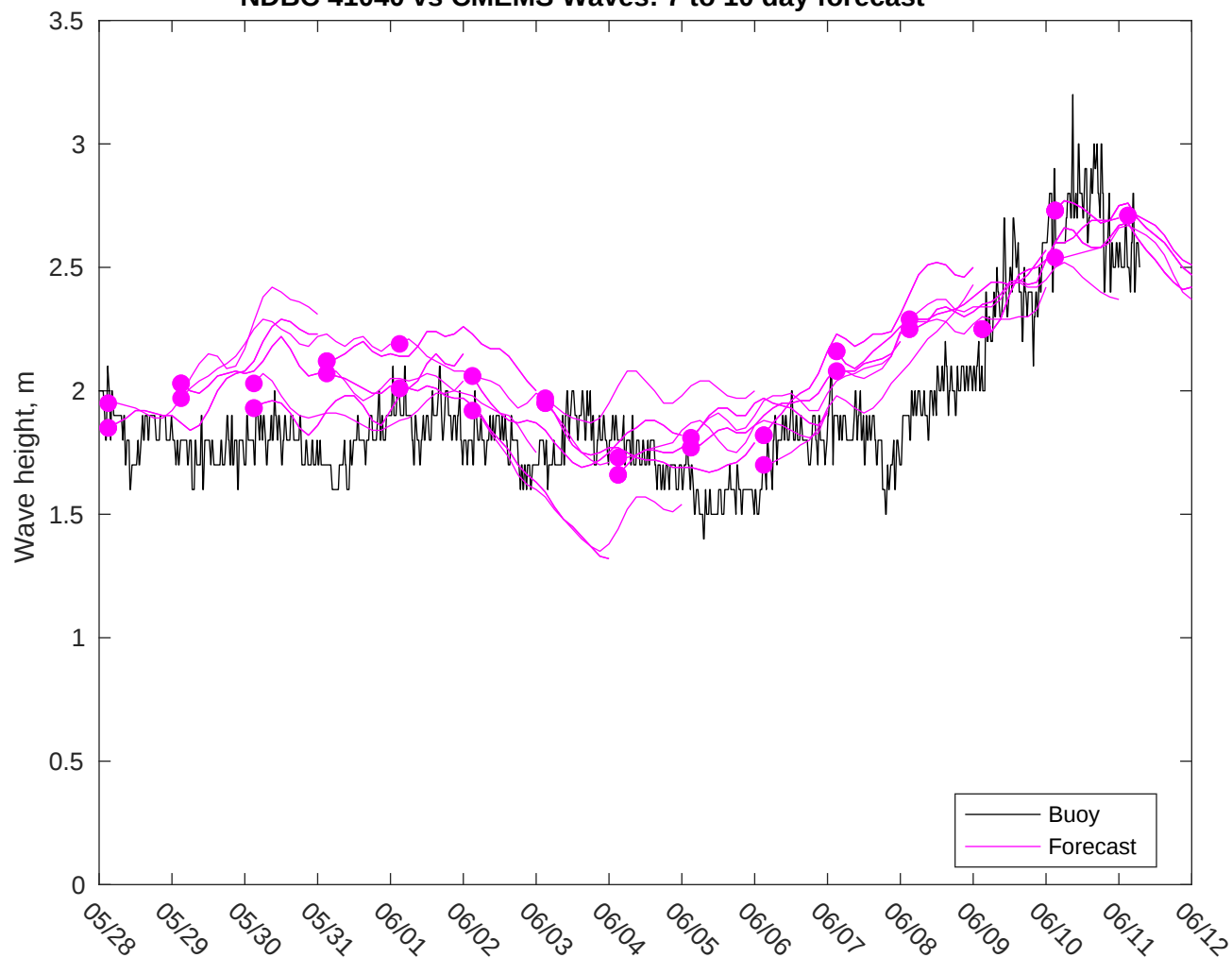
NDBC 41040 vs CMEMS Waves: 7 to 10 day forecast
