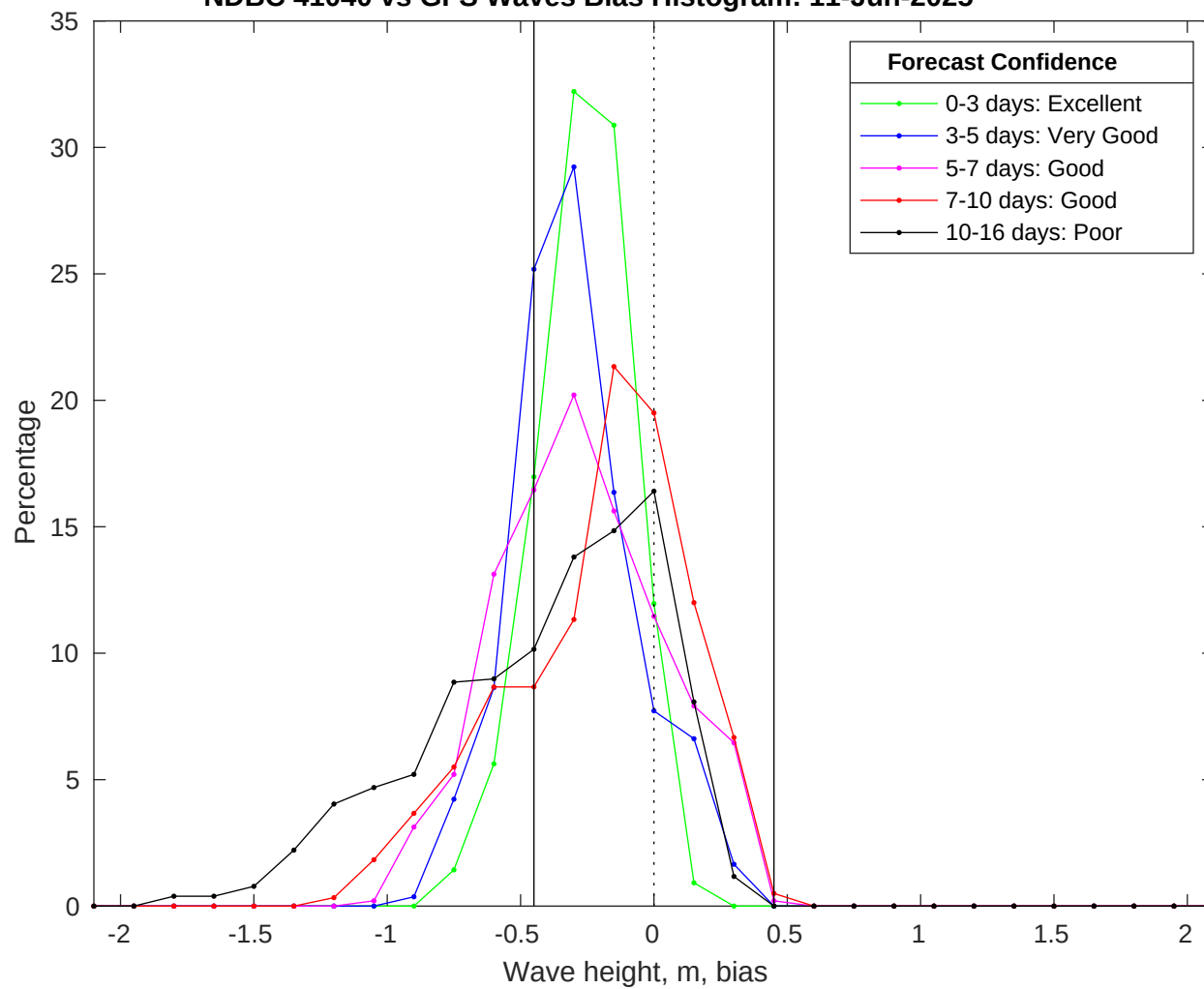
NDBC 41040 vs GFS Waves Bias Histogram: 11-Jun-2025
