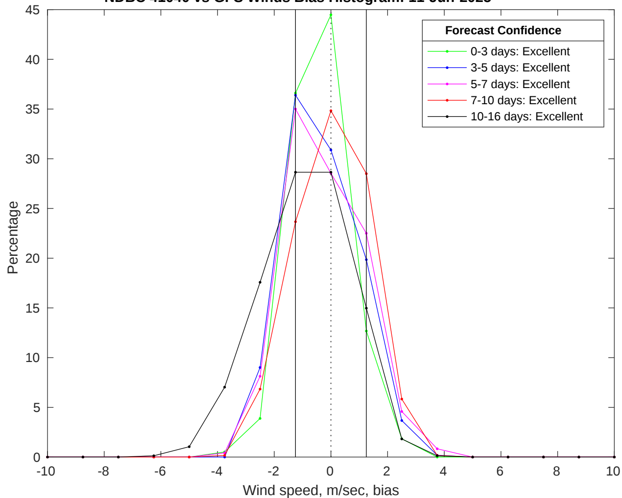
NDBC 41040 vs GFS Winds Bias Histogram: 11-Jun-2025
