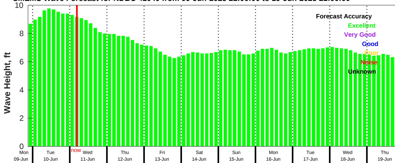
CMEMS Wave Forecast for NDBC 41040 from 09-Jun-2025 21:00:00 to 19-Jun-2025 21:00:00
