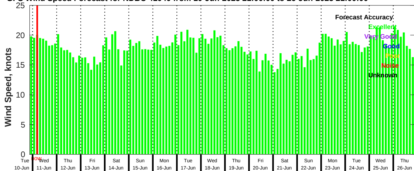
GFS Wind Speed Forecast for NDBC 41040 from 10-Jun-2025 21:00:00 to 26-Jun-2025 21:00:00
