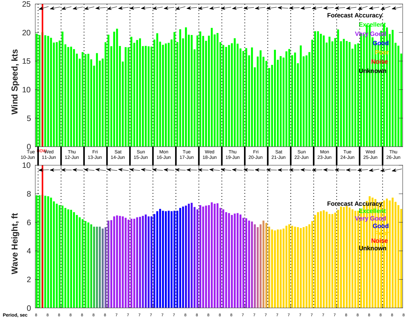
Wind & Wave Forecast for NDBC 41040 from 10-Jun-2025 21:00:00 to 26-Jun-2025 21:00:00
