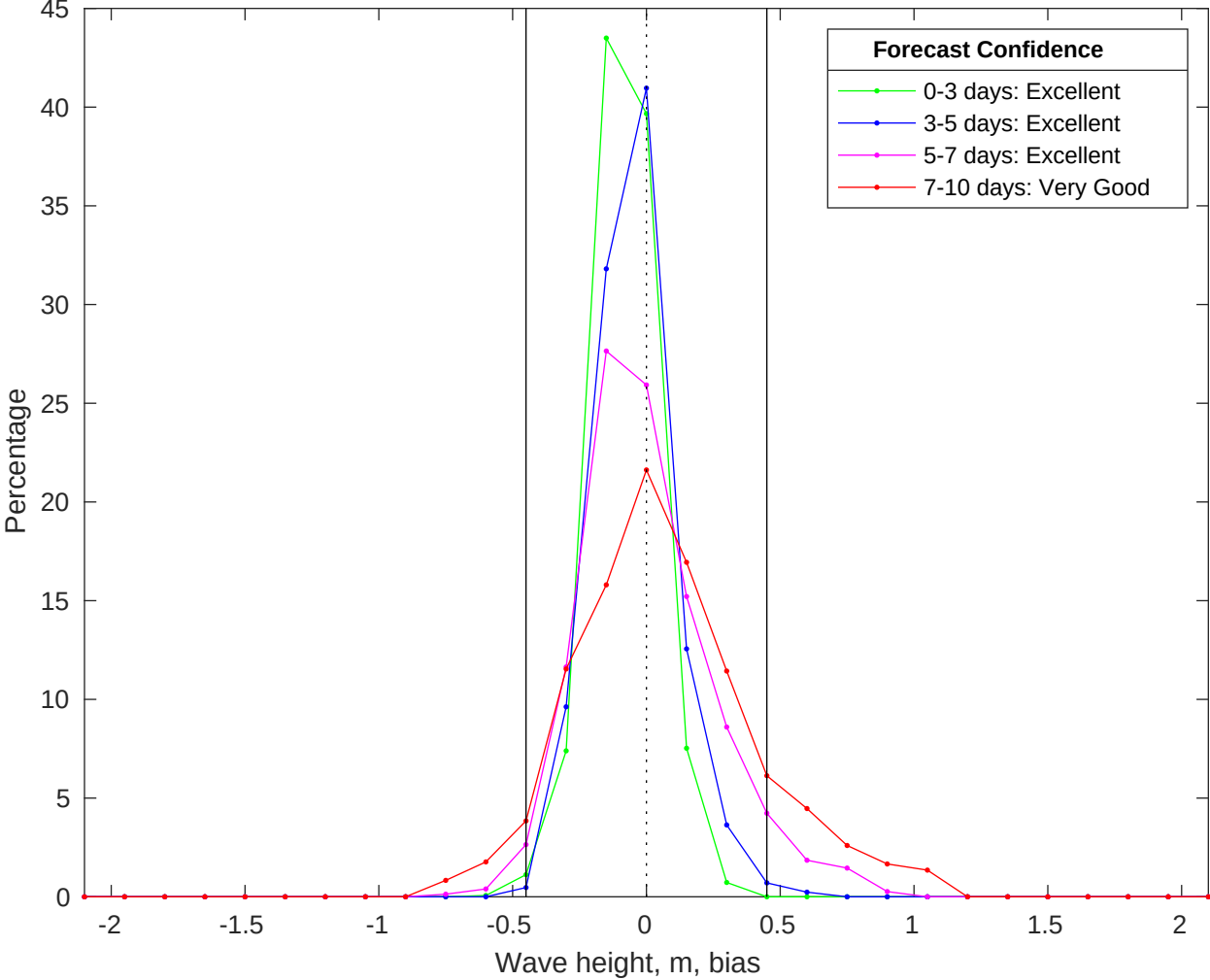
NDBC 42019 vs CMEMS Waves Bias Histogram: 11-Jun-2025
