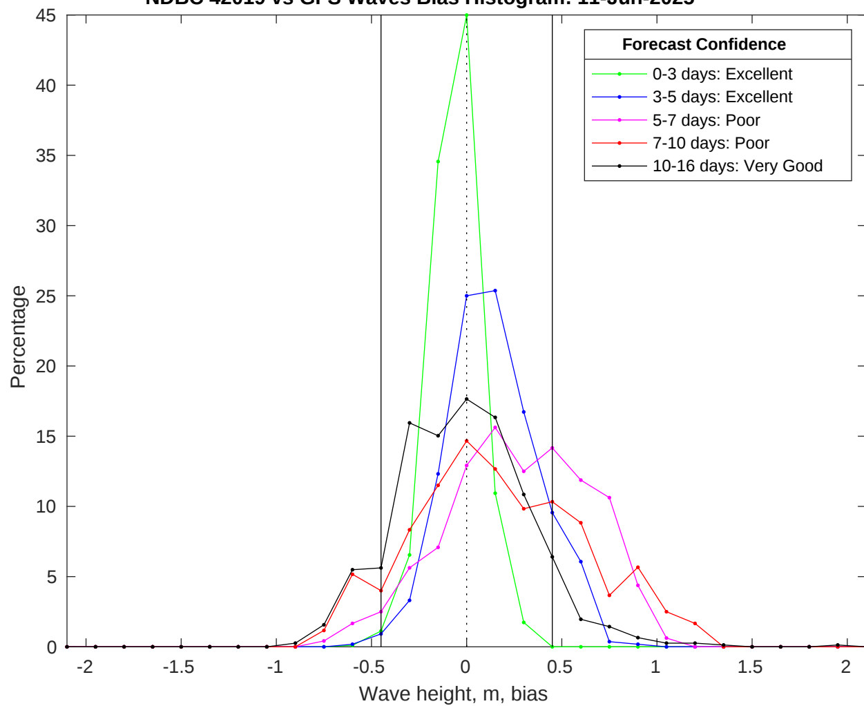
NDBC 42019 vs GFS Waves Bias Histogram: 11-Jun-2025
