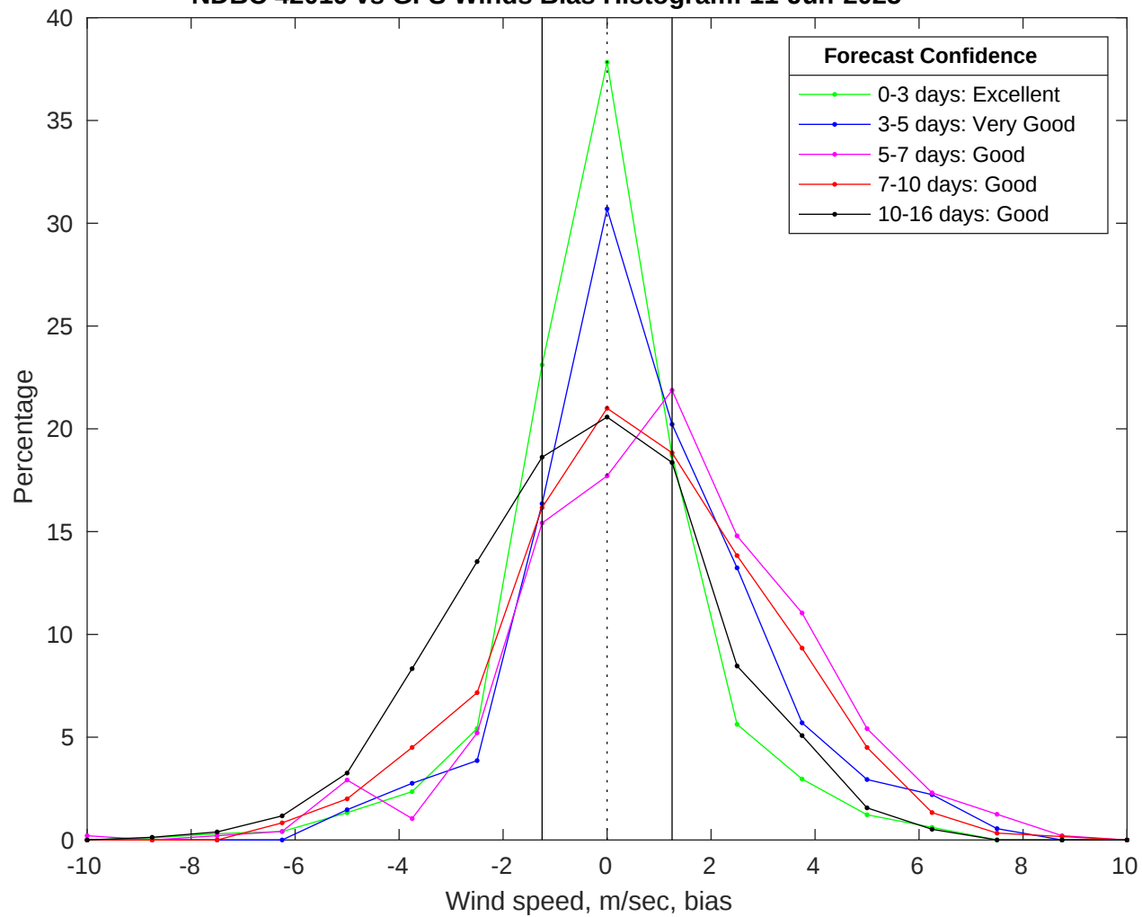
NDBC 42019 vs GFS Winds Bias Histogram: 11-Jun-2025
