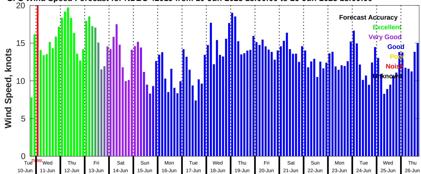
GFS Wind Speed Forecast for NDBC 42019 from 10-Jun-2025 18:00:00 to 26-Jun-2025 18:00:00
