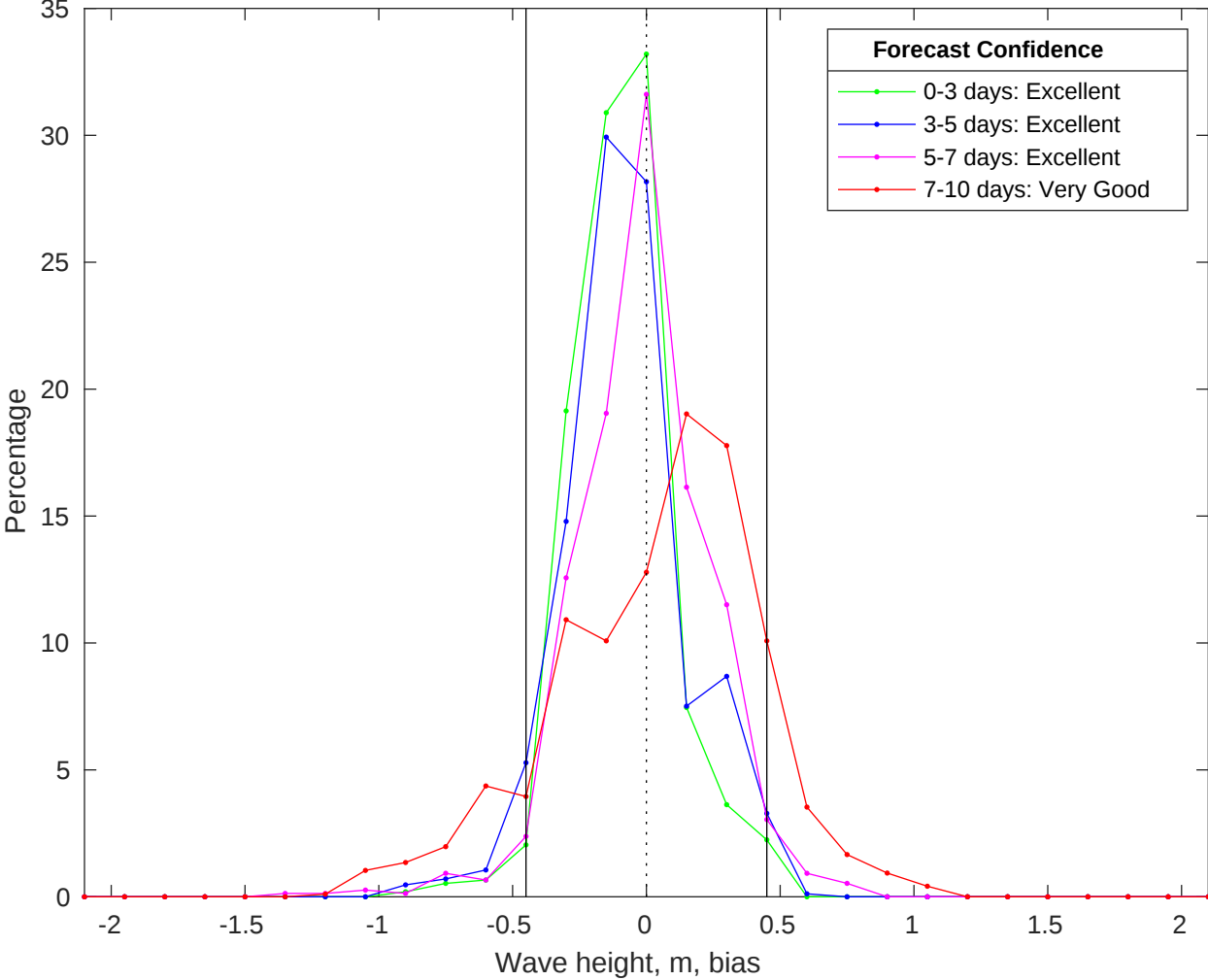
NDBC 42020 vs CMEMS Waves Bias Histogram: 11-Jun-2025
