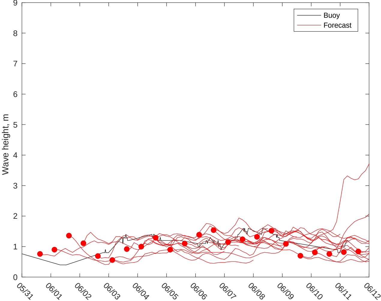
NDBC 42020 vs GFS Waves: 10 to 16 day forecast
