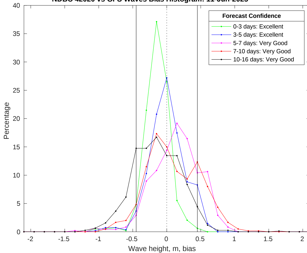
NDBC 42020 vs GFS Waves Bias Histogram: 11-Jun-2025
