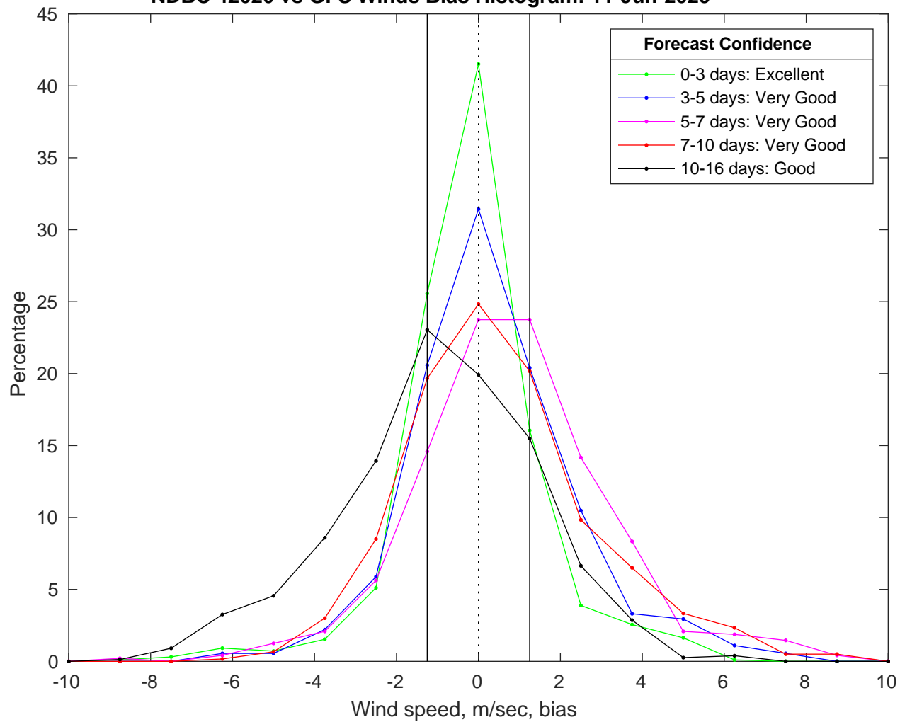
NDBC 42020 vs GFS Winds Bias Histogram: 11-Jun-2025
