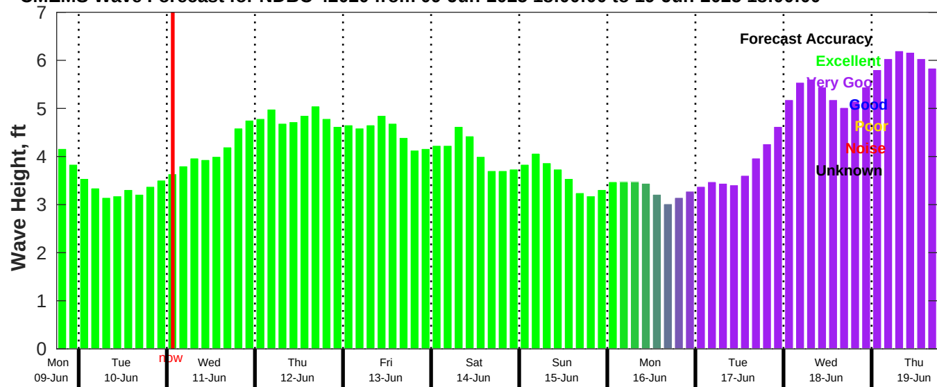
CMEMS Wave Forecast for NDBC 42020 from 09-Jun-2025 18:00:00 to 19-Jun-2025 18:00:00
