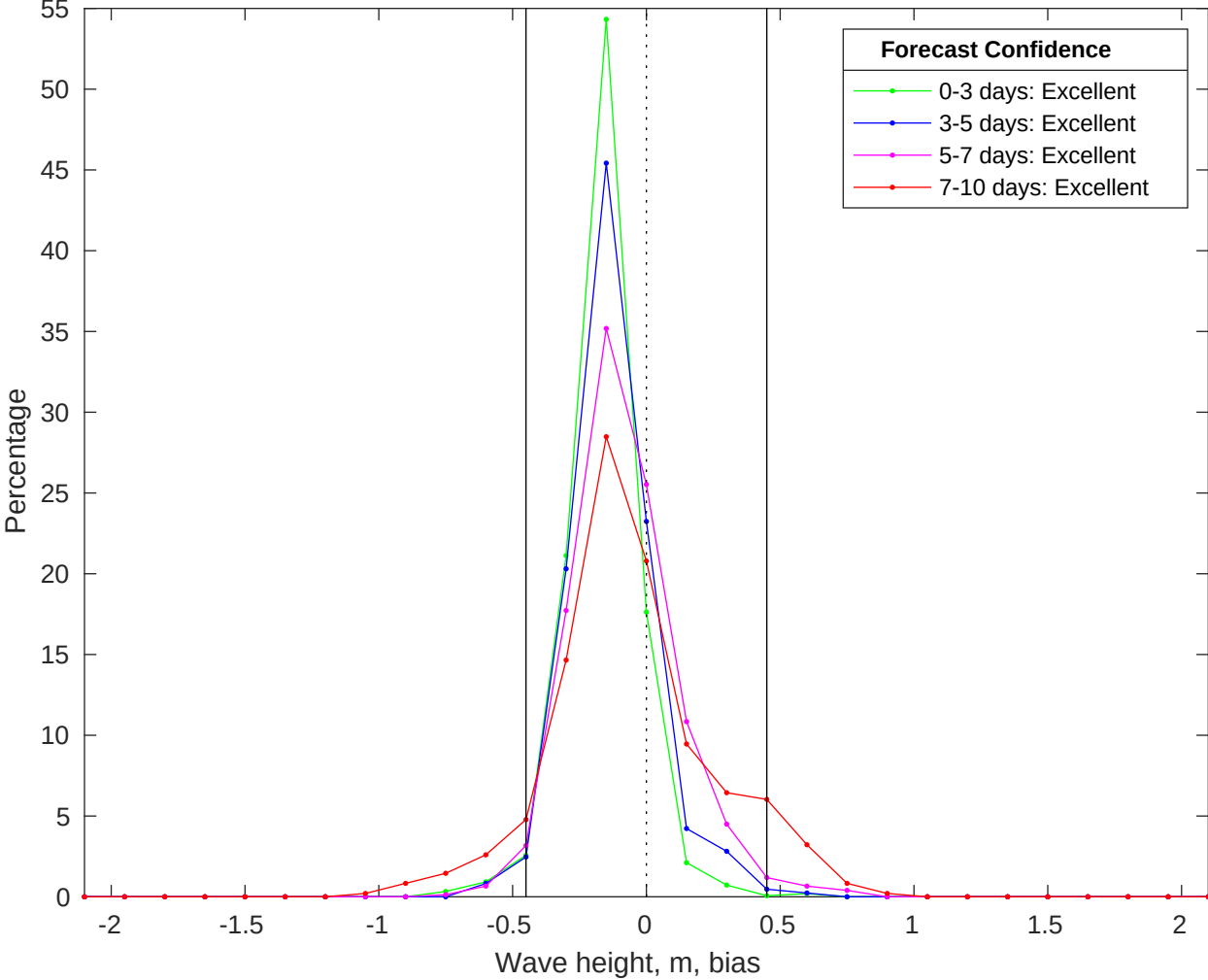
NDBC 42035 vs CMEMS Waves Bias Histogram: 11-Jun-2025
