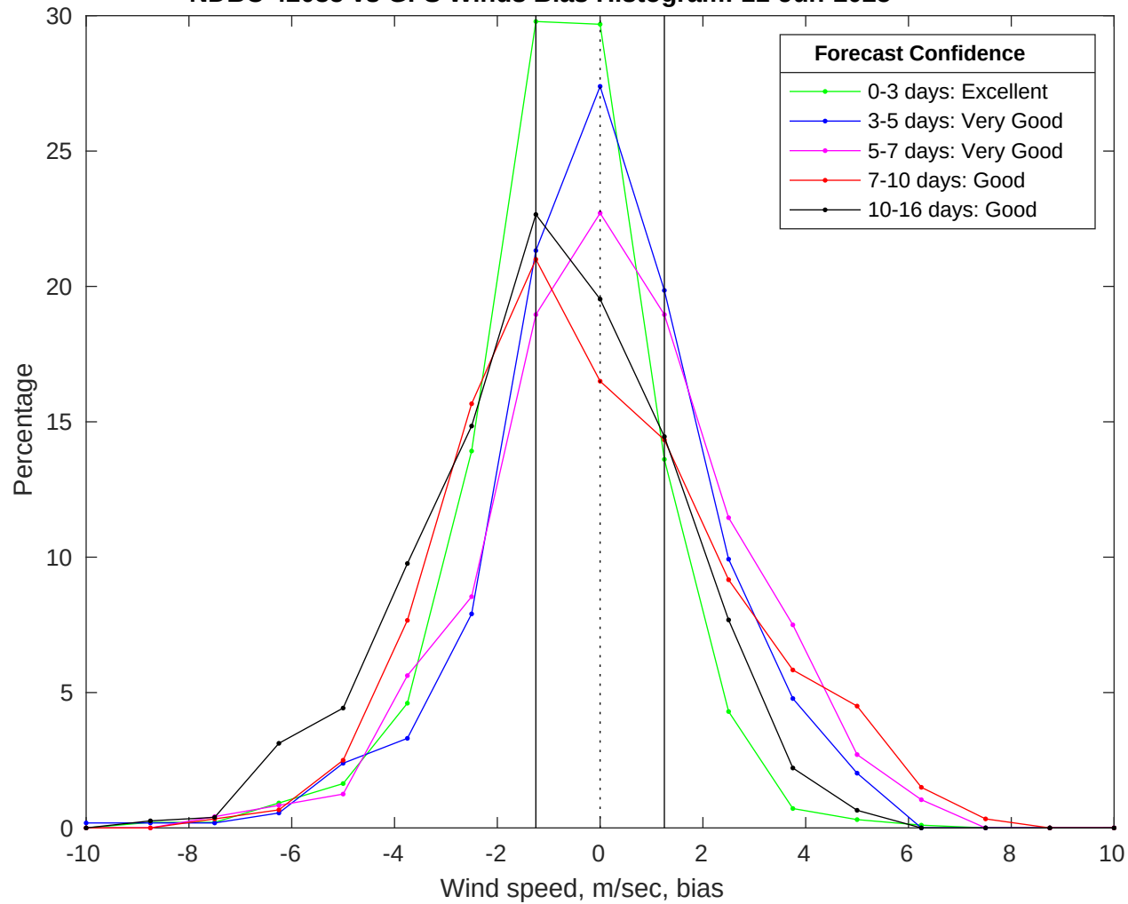
NDBC 42035 vs GFS Winds Bias Histogram: 11-Jun-2025
