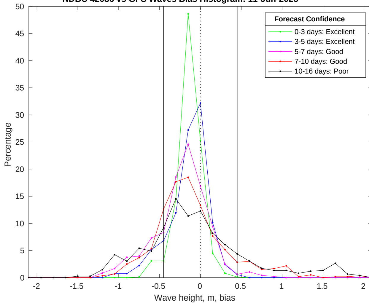
NDBC 42036 vs GFS Waves Bias Histogram: 11-Jun-2025
