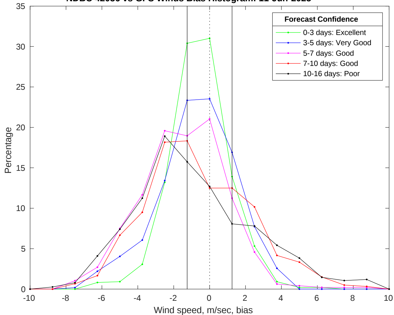
NDBC 42036 vs GFS Winds Bias Histogram: 11-Jun-2025
