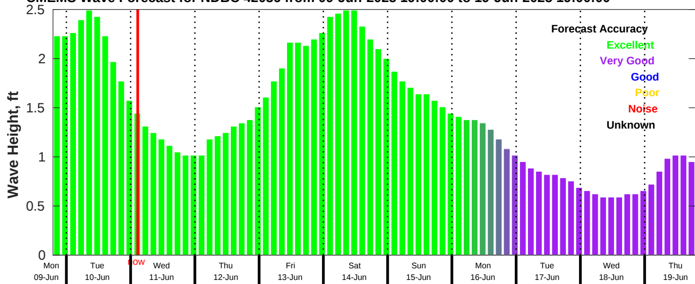
CMEMS Wave Forecast for NDBC 42036 from 09-Jun-2025 19:00:00 to 19-Jun-2025 19:00:00
