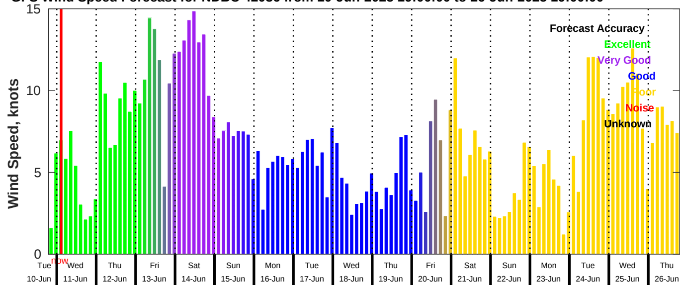
GFS Wind Speed Forecast for NDBC 42036 from 10-Jun-2025 19:00:00 to 26-Jun-2025 19:00:00
