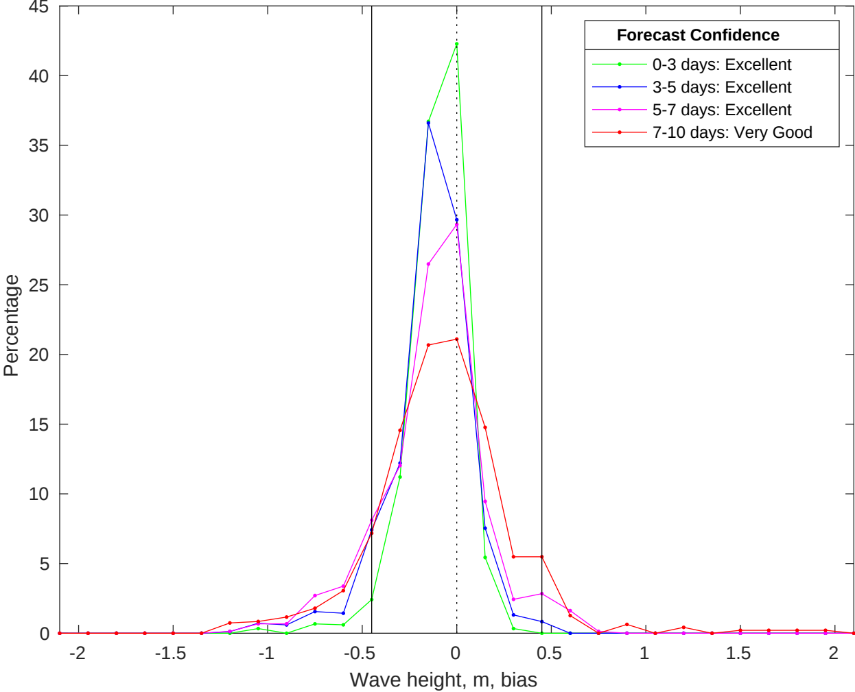
NDBC 42040 vs CMEMS Waves Bias Histogram: 11-Jun-2025
