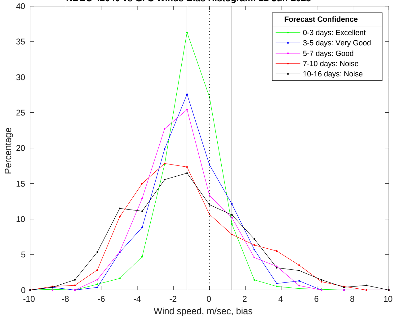
NDBC 42040 vs GFS Winds Bias Histogram: 11-Jun-2025
