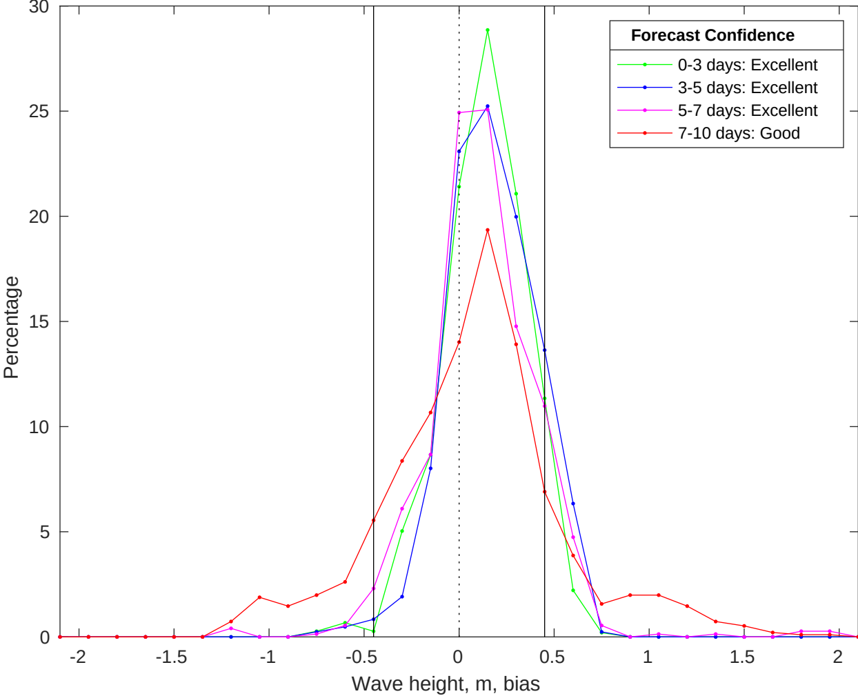
NDBC 46011 vs CMEMS Waves Bias Histogram: 11-Jun-2025
