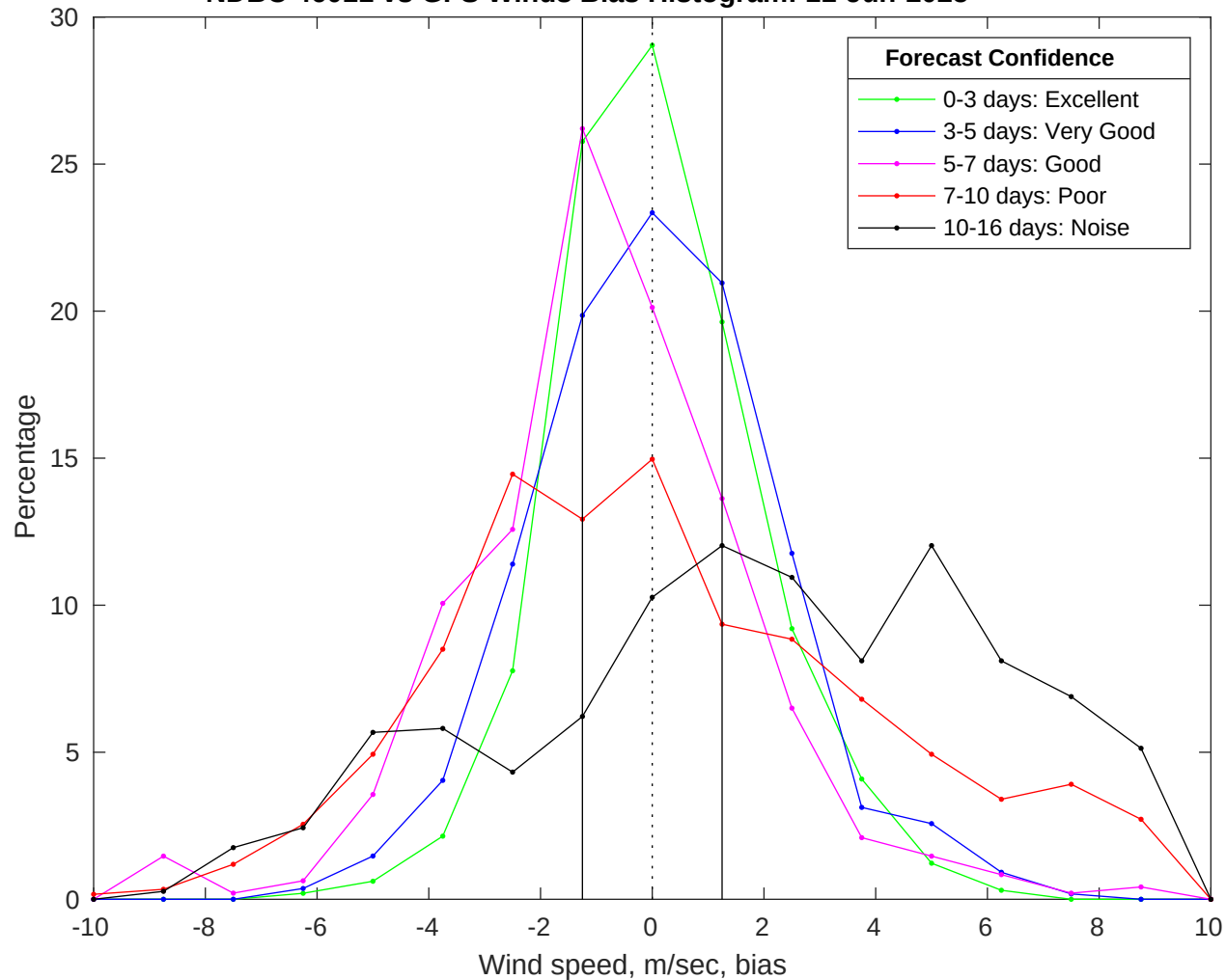
NDBC 46011 vs GFS Winds Bias Histogram: 11-Jun-2025
