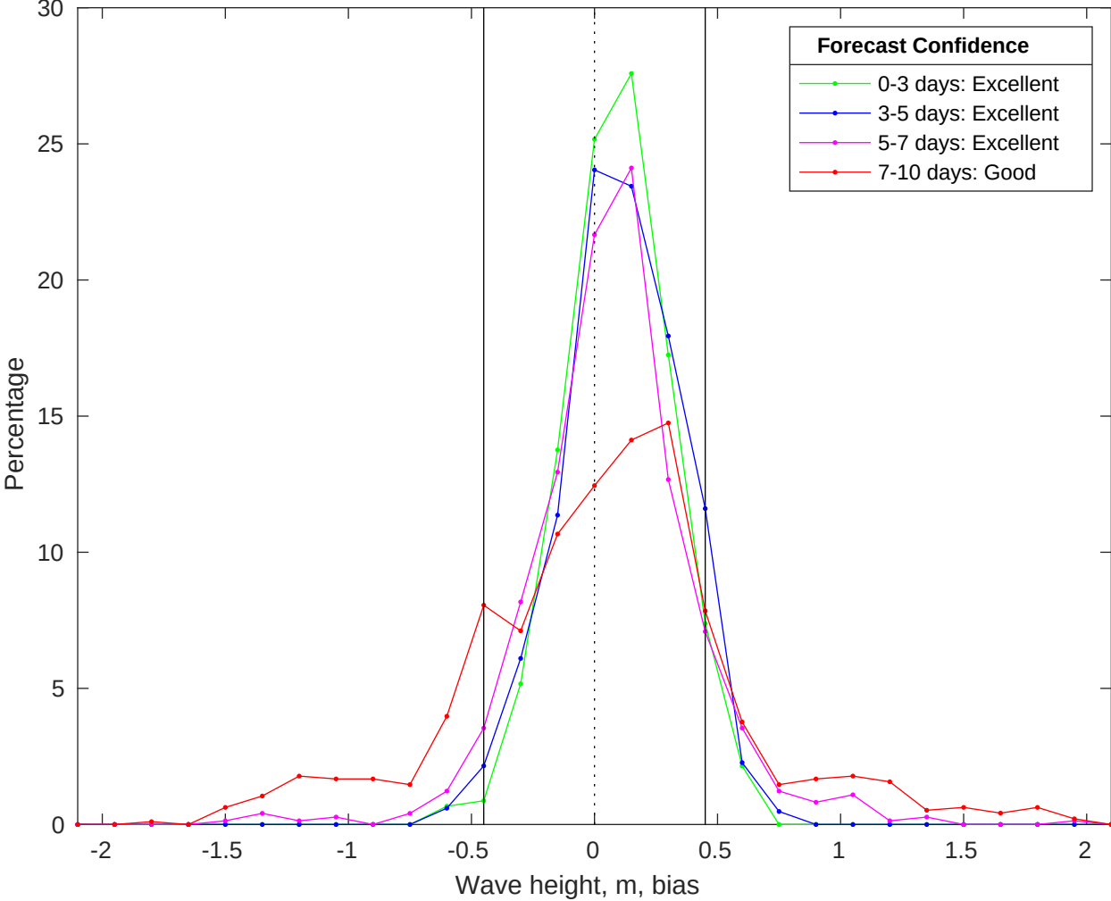
NDBC 46028 vs CMEMS Waves Bias Histogram: 11-Jun-2025
