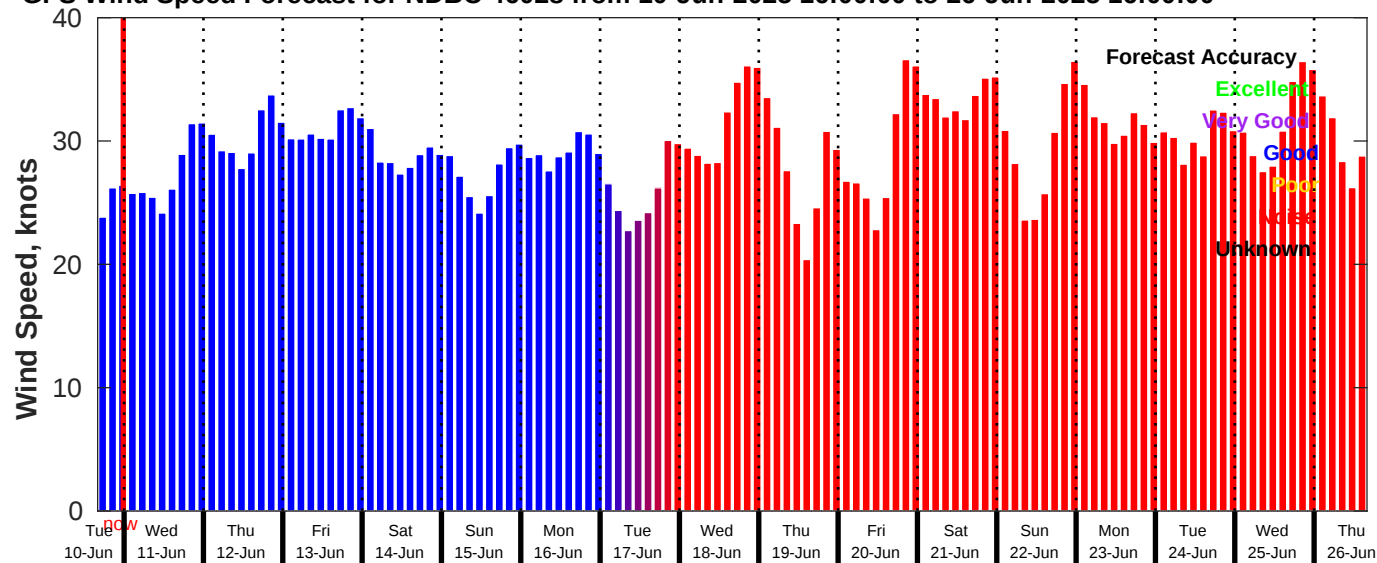
GFS Wind Speed Forecast for NDBC 46028 from 10-Jun-2025 16:00:00 to 26-Jun-2025 16:00:00
