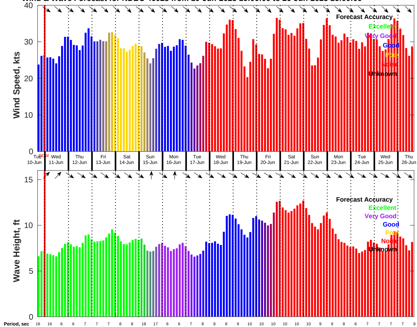
Wind & Wave Forecast for NDBC 46028 from 10-Jun-2025 16:00:00 to 26-Jun-2025 16:00:00
