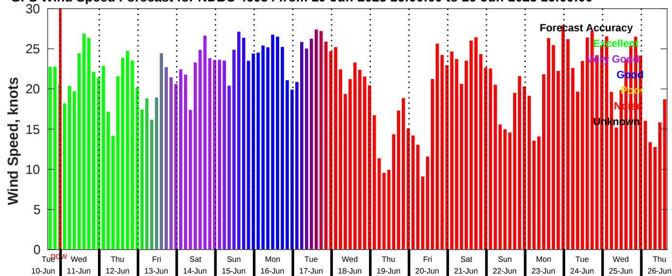
GFS Wind Speed Forecast for NDBC 46054 from 10-Jun-2025 16:00:00 to 26-Jun-2025 16:00:00
