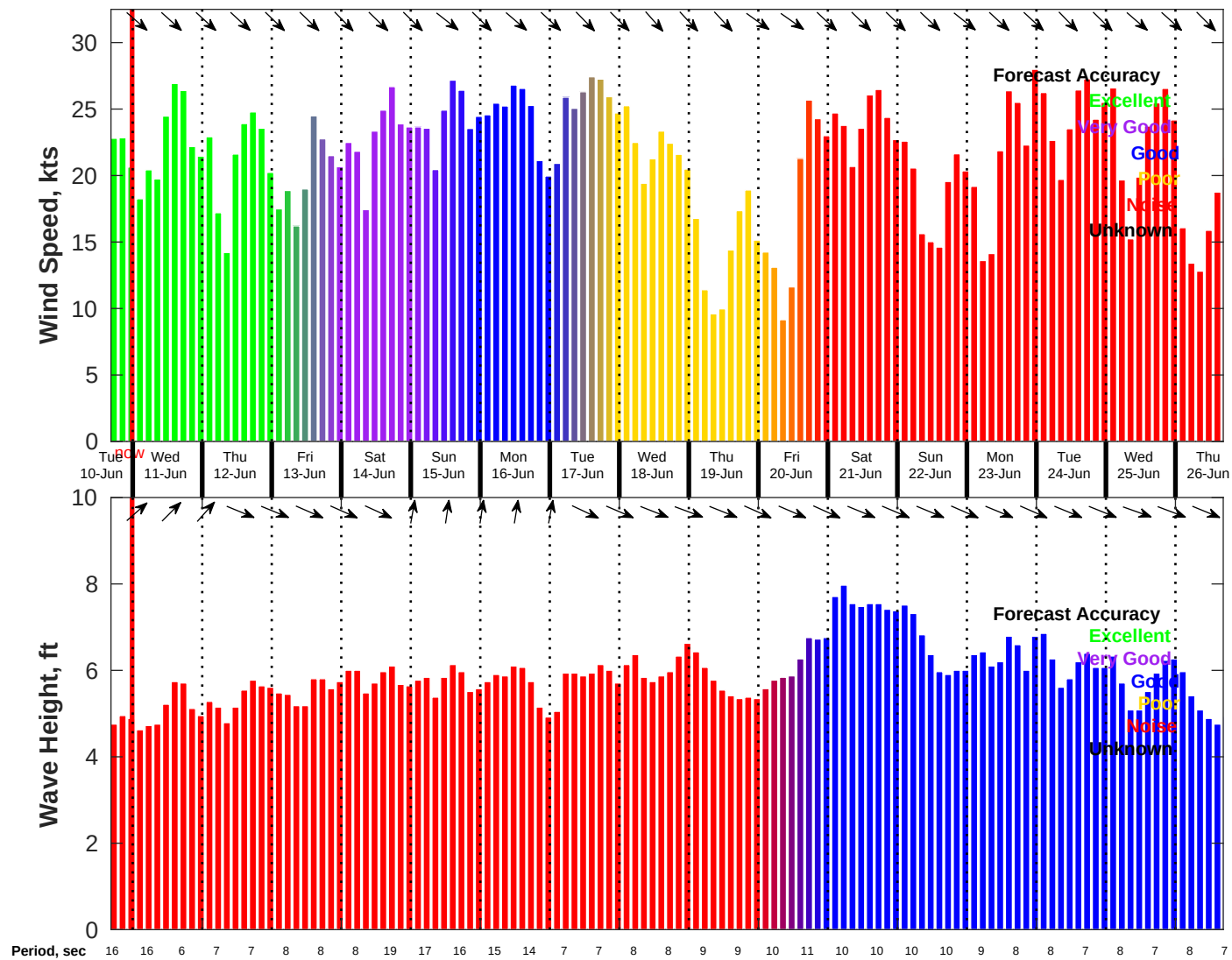
Wind & Wave Forecast for NDBC 46054 from 10-Jun-2025 16:00:00 to 26-Jun-2025 16:00:00
