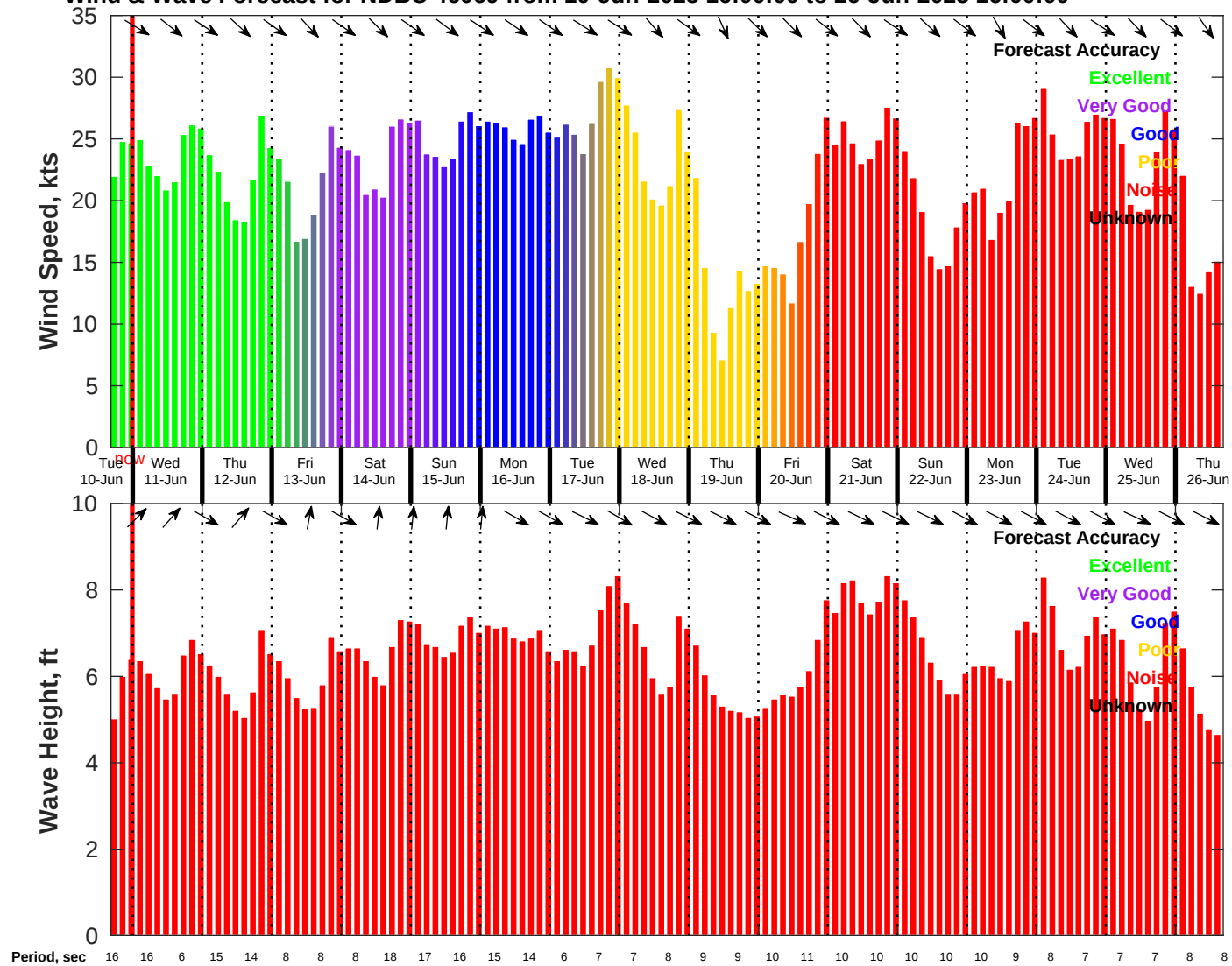
Wind & Wave Forecast for NDBC 46069 from 10-Jun-2025 16:00:00 to 26-Jun-2025 16:00:00
