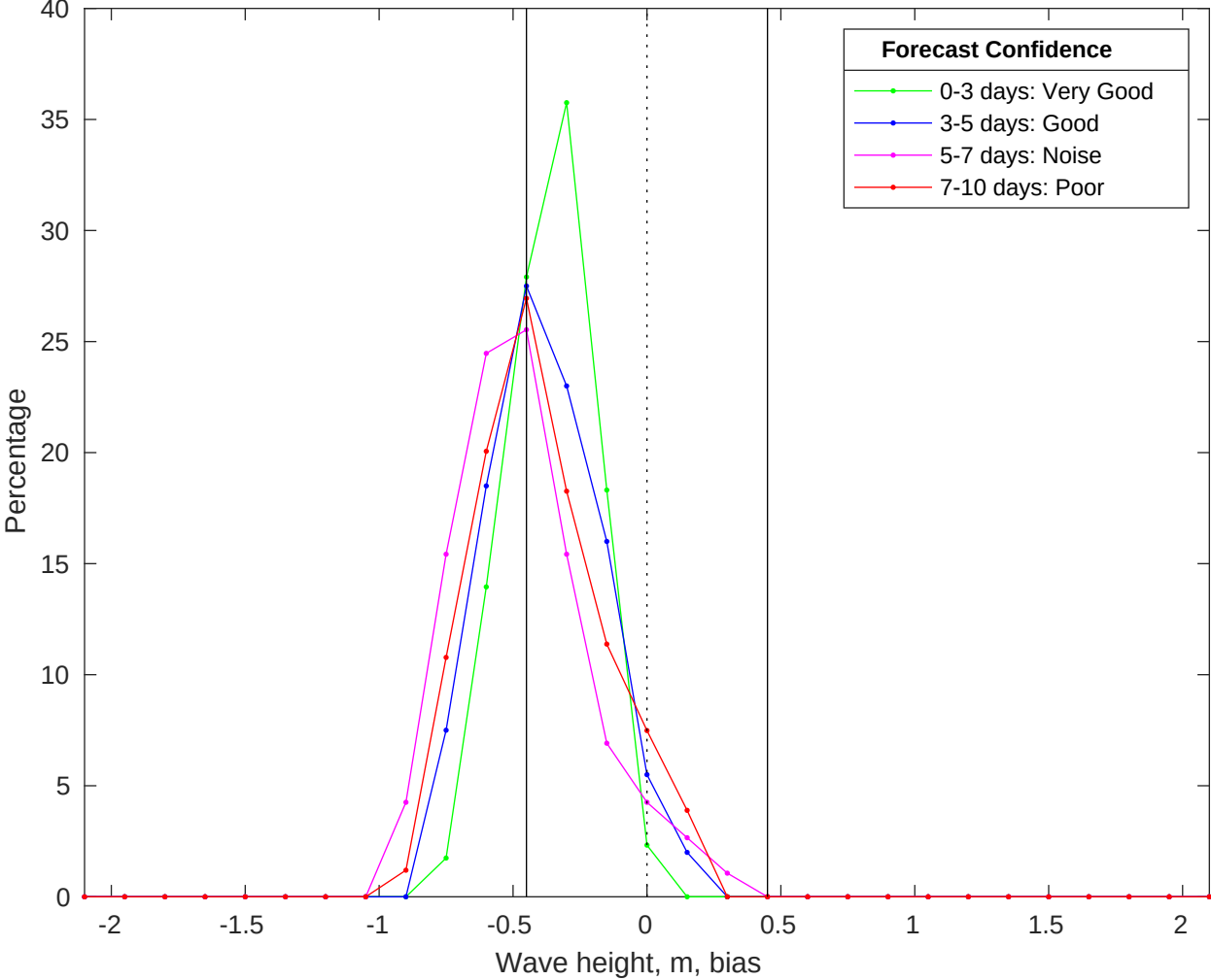
NDBC 51209 vs CMEMS Waves Bias Histogram: 11-Jun-2025
