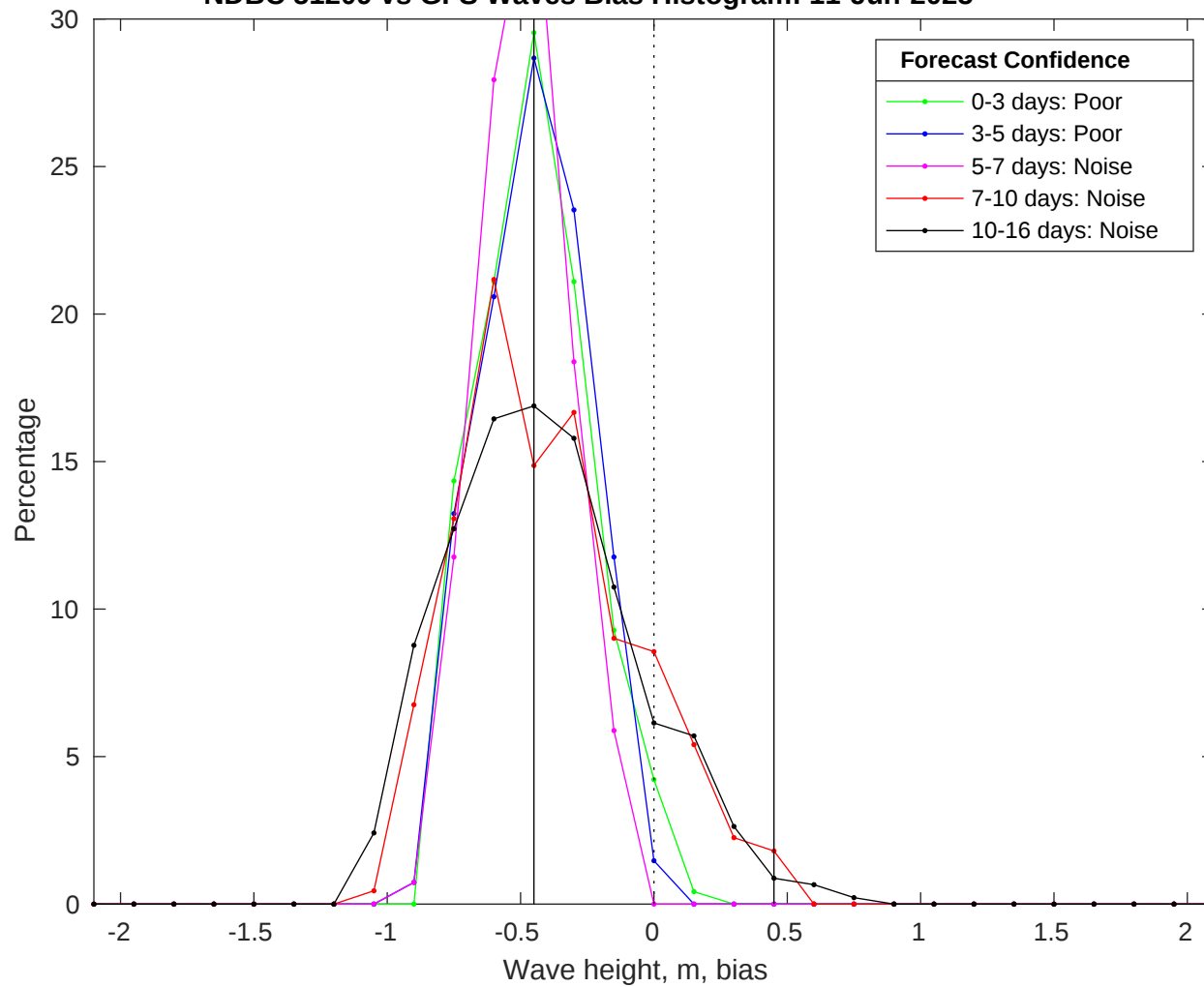
NDBC 51209 vs GFS Waves Bias Histogram: 11-Jun-2025
