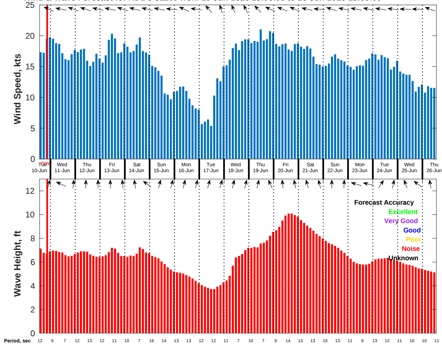
Wind & Wave Forecast for NDBC 51209 from 10-Jun-2025 13:00:00 to 26-Jun-2025 13:00:00
