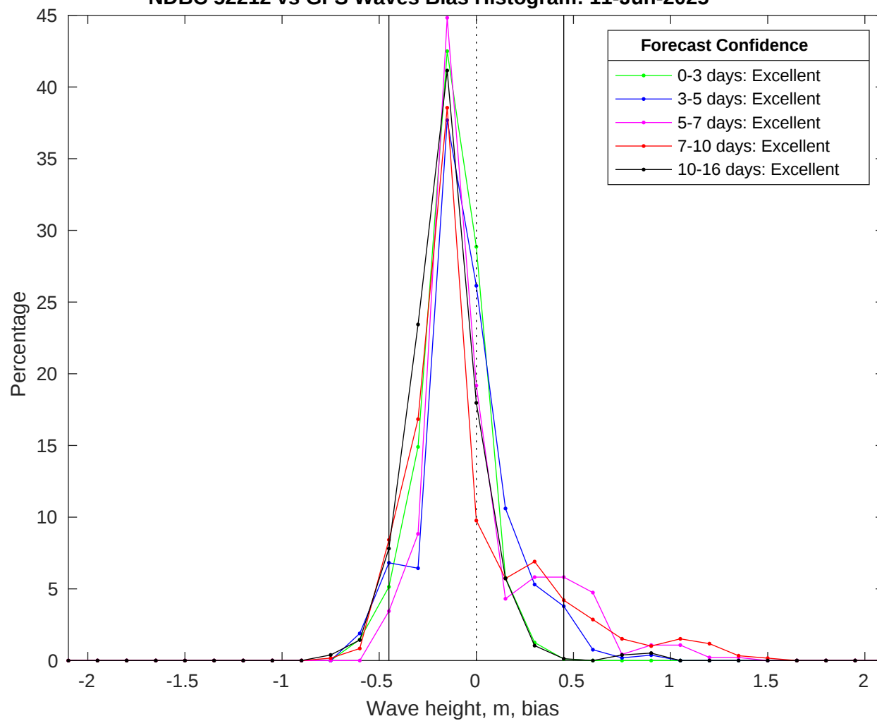
NDBC 52212 vs GFS Waves Bias Histogram: 11-Jun-2025
