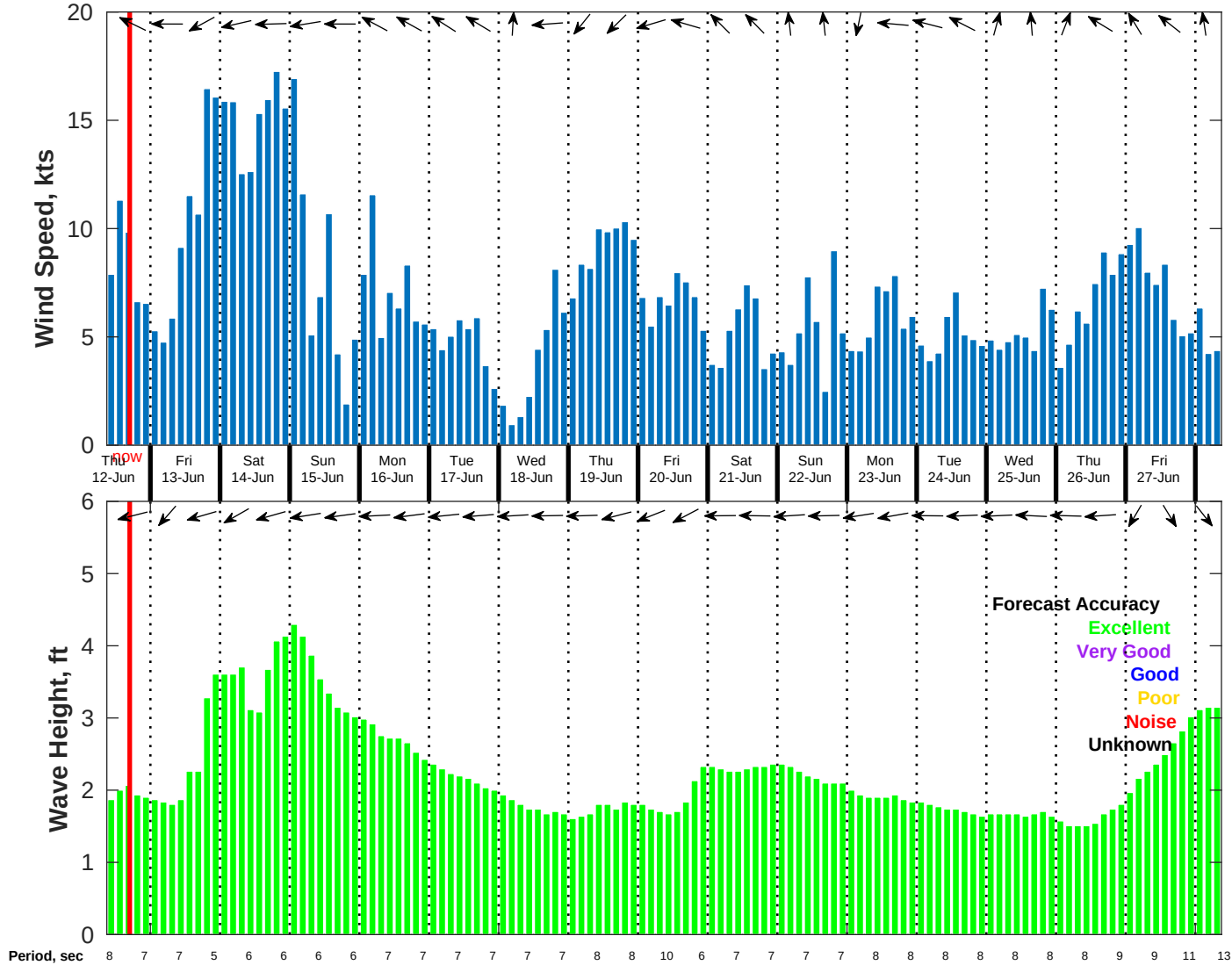
Wind & Wave Forecast for NDBC 52212 from 11-Jun-2025 09:00:00 to 27-Jun-2025 09:00:00
