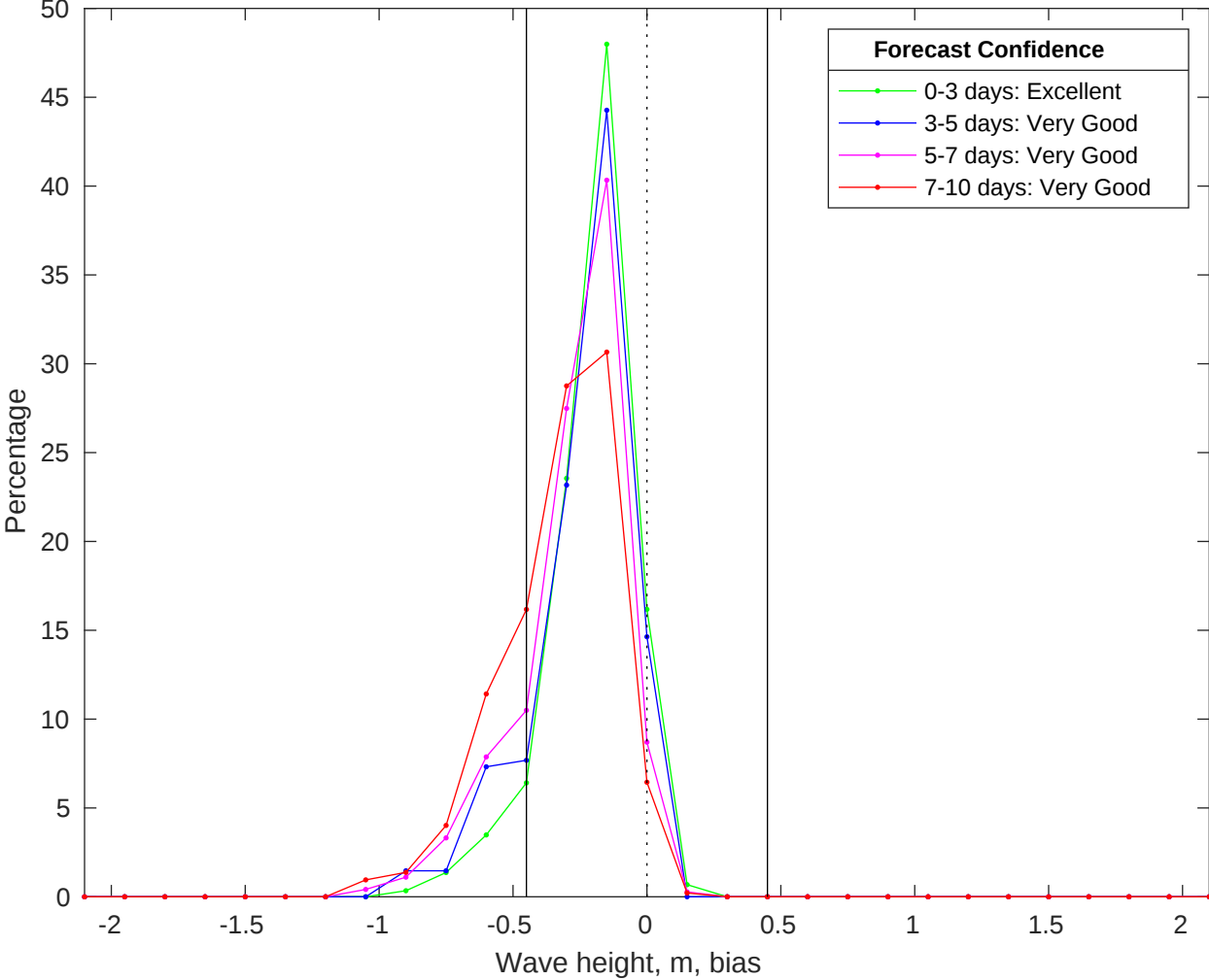
NDBC 52213 vs CMEMS Waves Bias Histogram: 11-Jun-2025
