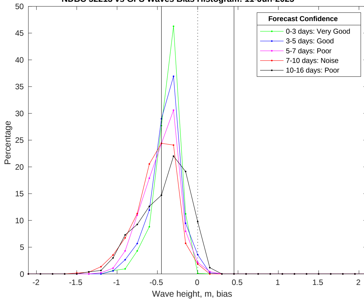
NDBC 52213 vs GFS Waves Bias Histogram: 11-Jun-2025
