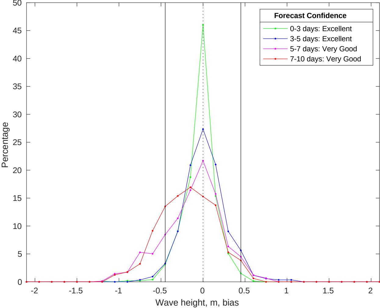
NDBC 41004 vs CMEMS Waves Bias Histogram: 12-Jun-2025
