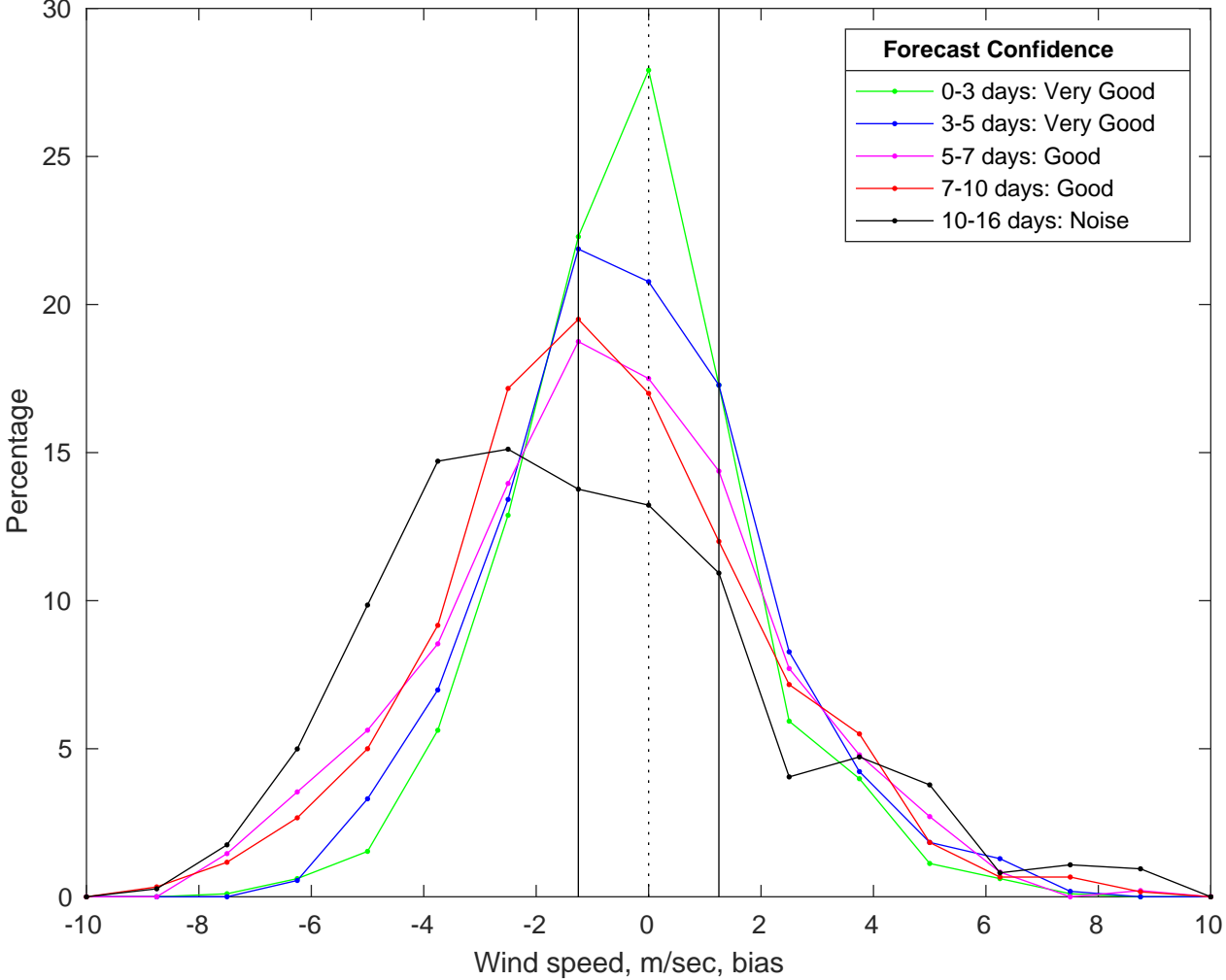
NDBC 41004 vs GFS Winds Bias Histogram: 12-Jun-2025
