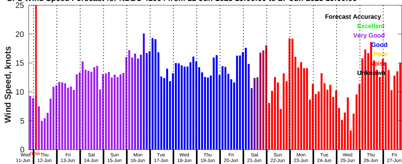
GFS Wind Speed Forecast for NDBC 41004 from 11-Jun-2025 19:00:00 to 27-Jun-2025 19:00:00
