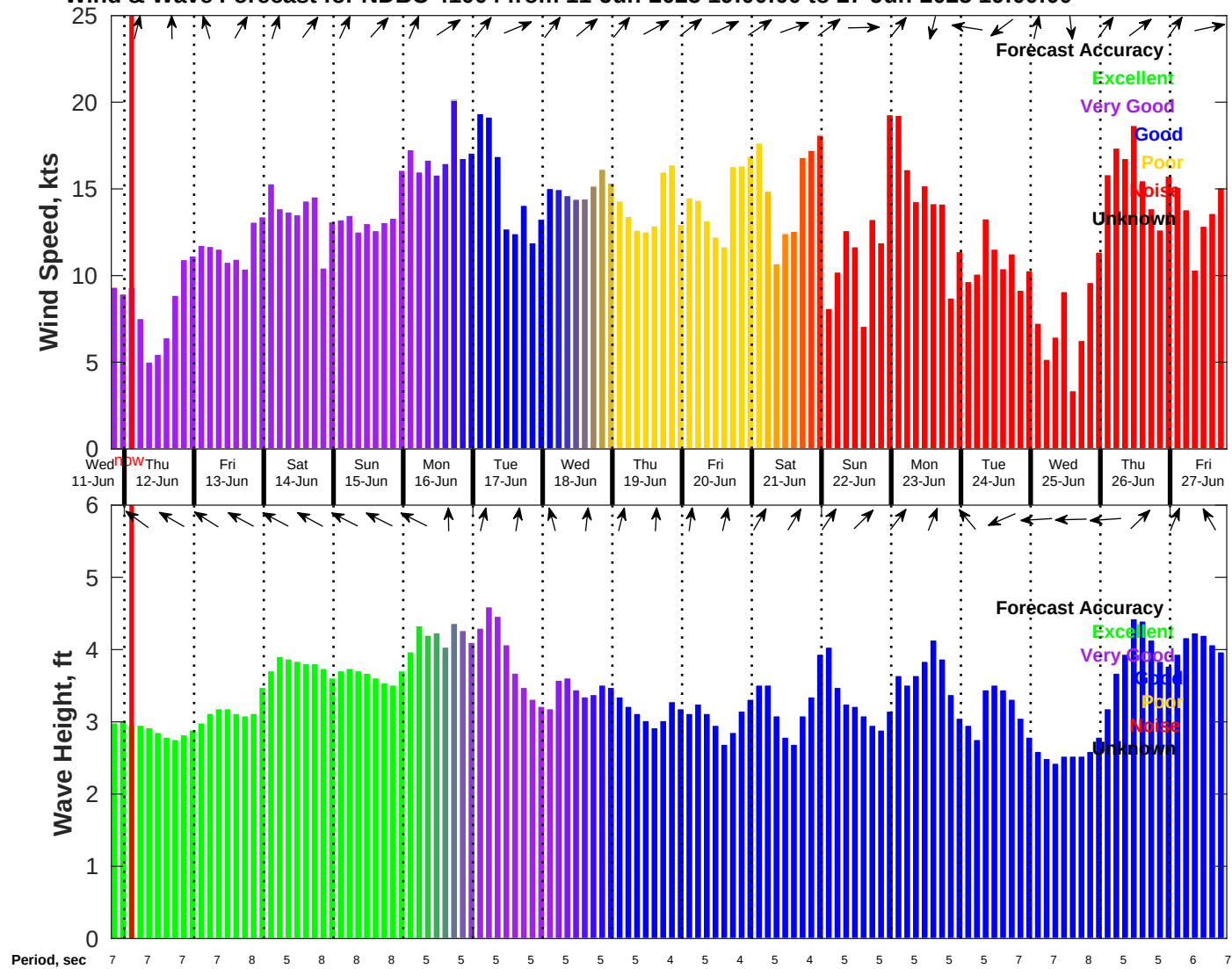
Wind & Wave Forecast for NDBC 41004 from 11-Jun-2025 19:00:00 to 27-Jun-2025 19:00:00
