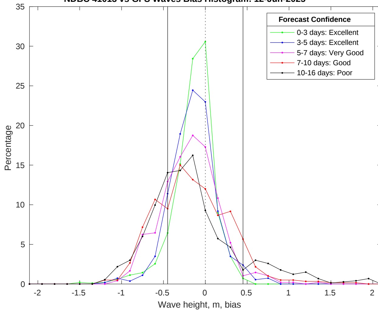
NDBC 41013 vs GFS Waves Bias Histogram: 12-Jun-2025
