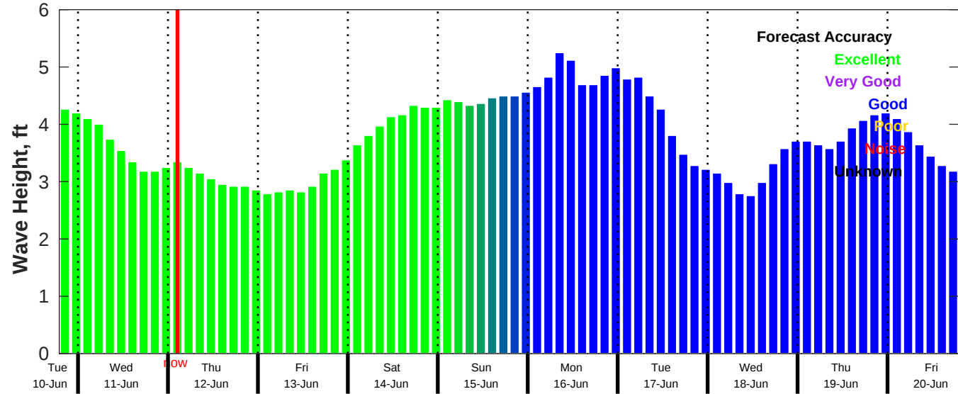
CMEMS Wave Forecast for NDBC 41013 from 10-Jun-2025 19:00:00 to 20-Jun-2025 19:00:00
