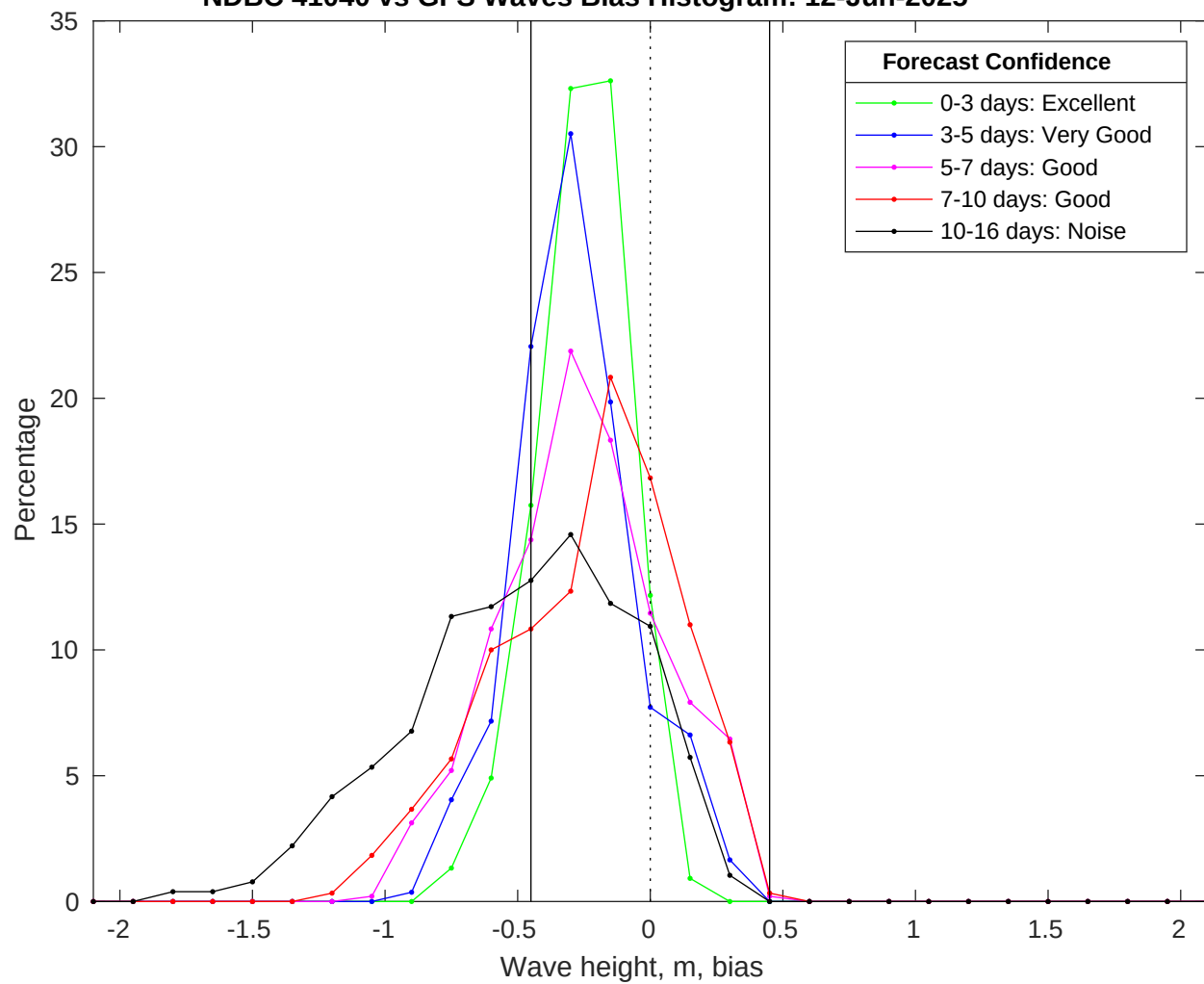
NDBC 41040 vs GFS Waves Bias Histogram: 12-Jun-2025
