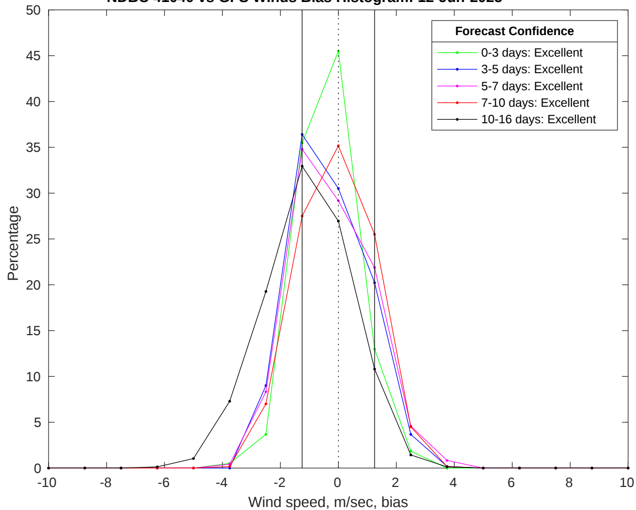
NDBC 41040 vs GFS Winds Bias Histogram: 12-Jun-2025
