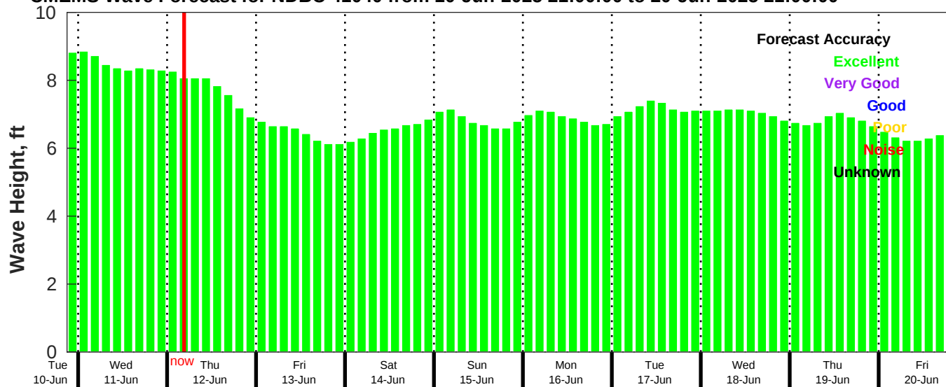
CMEMS Wave Forecast for NDBC 41040 from 10-Jun-2025 21:00:00 to 20-Jun-2025 21:00:00
