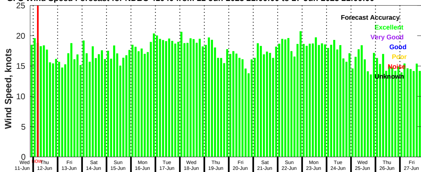
GFS Wind Speed Forecast for NDBC 41040 from 11-Jun-2025 21:00:00 to 27-Jun-2025 21:00:00
